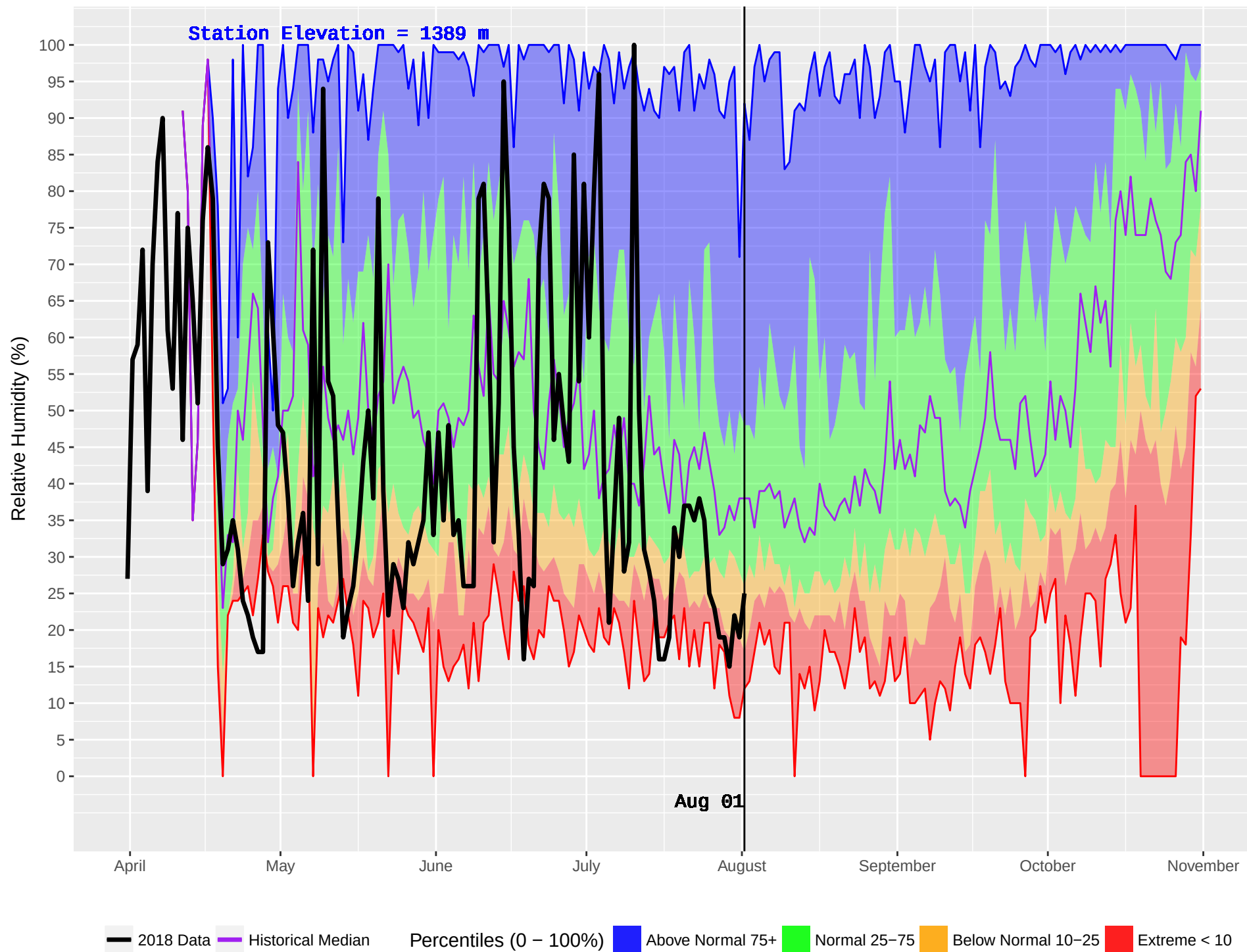
KETTLE 2 (388) : Historical (1987–2016) and Current (2018) Daily Relative Humidity
