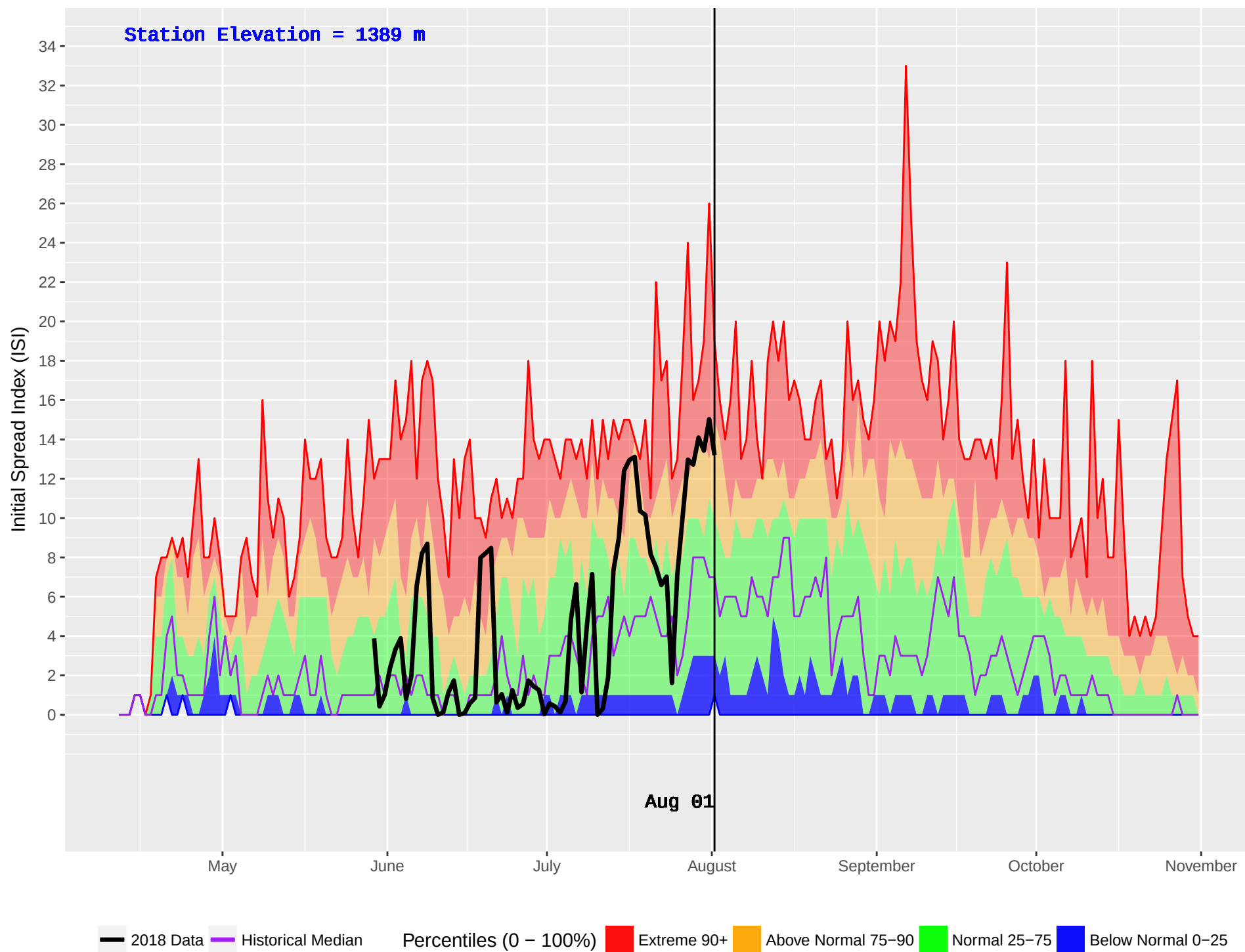
KETTLE 2 (388) : Historical (1987–2016) and Current (2018) Daily Initial Spread Index (ISI)
